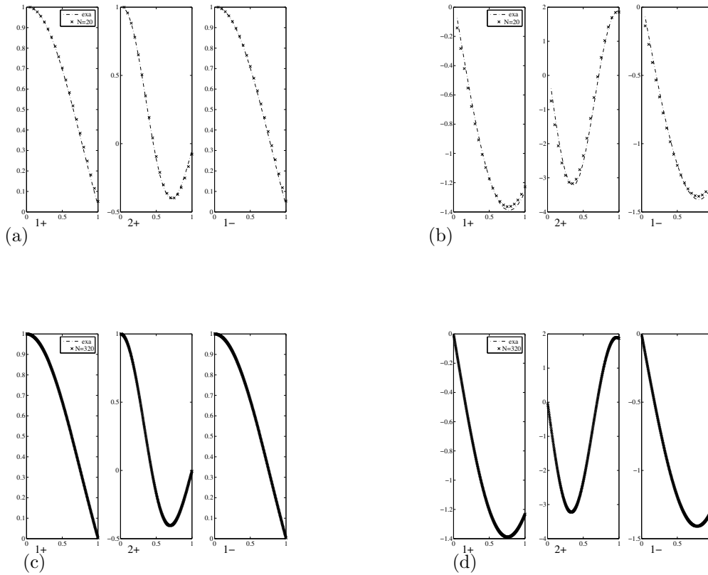
FIG. 3. (a) Temperature field T(i/n) i \in \{1, n\} for discretization n = 20 and Pe = 0.1 with the first two downstream eigenvectors 1+ and 2+ and the first upstream eigenvector 1- . Normalization T(0) = 1 has been imposed. (b) Temperature gradient p = \partial_r T(i/n)/\lambda for discretization n = 20 and Pe = 0.1 . (c) Same convention as (a) for discretization n = 320 . (d) Same convention as (b) for discretization n = 320 .
