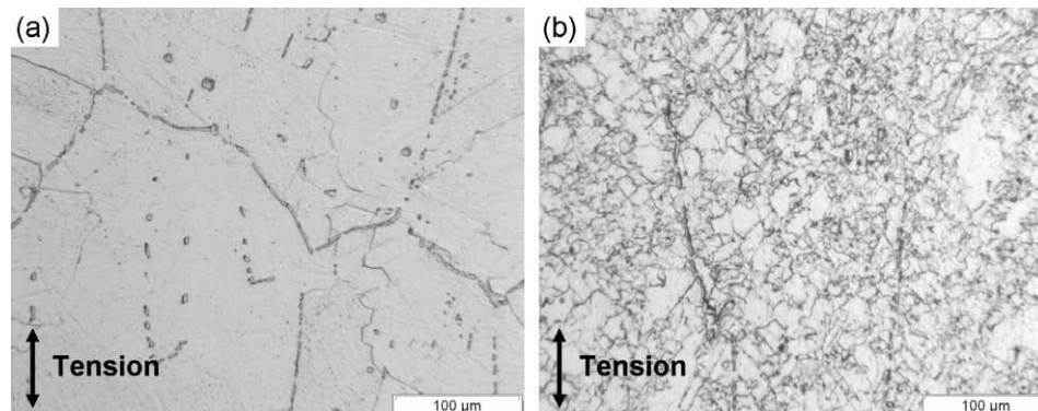
Fig. 10. Microstructure of the 1000 h/950 °C aged Inconel 617 creep sample after rupture at 950 °C under 35 MPa: (a) low reduction in area far from the rupture zone, and (b) high reduction in area near the rupture zone.
