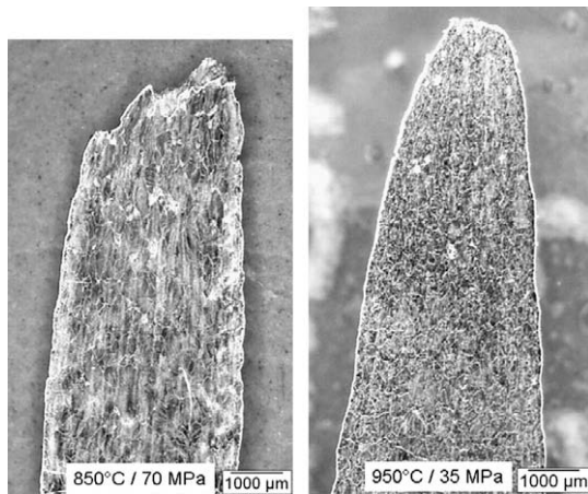
Fig. 7. Comparison of ruptured samples reduction in area between 850 °C/70 MPa and 950 °C/35 MPa.
