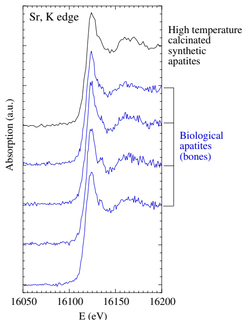
Fig. 7 XANES part of the absorption spectra near the Sr K edge for different bones compared to the XANES collected for a high-temperature-calcinated synthetic apatite
