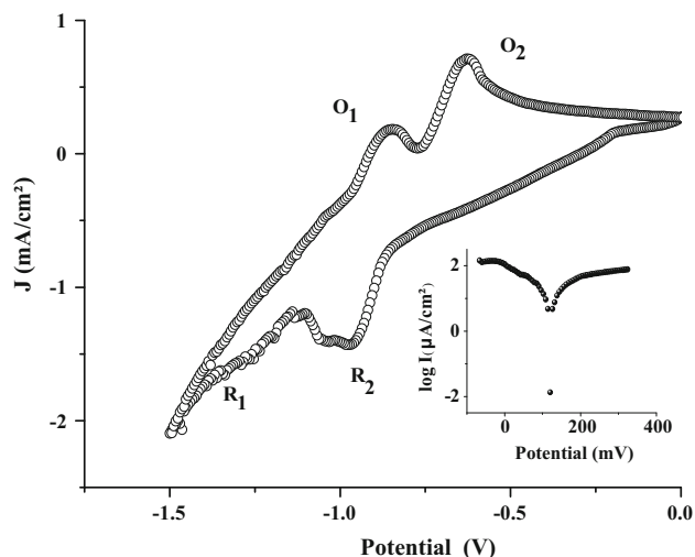
Fig. 9 Cyclic J (V) characteristic of \text{CuAlO}_2 in KOH solution (0.5 M) plotted under \text{N}_2 bubbling at 25^\circ\text{C} , scan rate 10 mV/s. Inset the semilogarithmic plot ( \log J -V)
