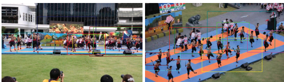
Figure 2: Bounding Boxes
