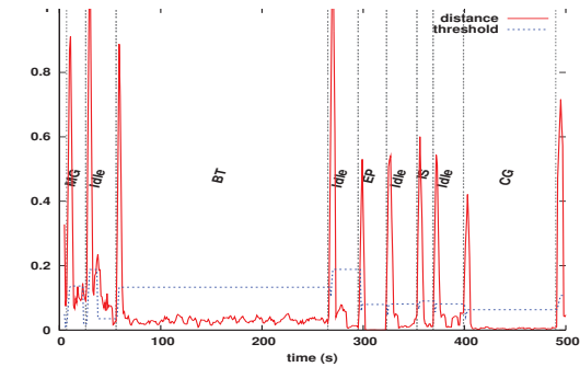
(c) Distance between EVs and variation of the detection threshold (master node.)
