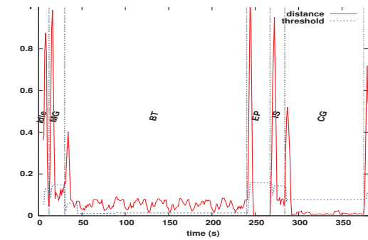
(c) Distance between EVs and variation of the detection threshold (master node).
