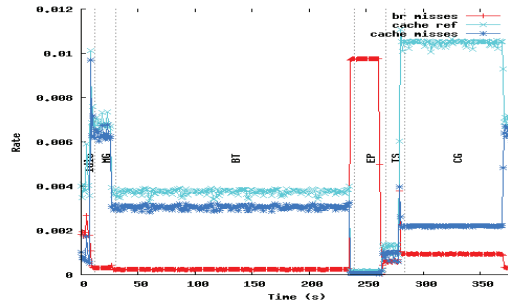
(b) Cache reference and miss rates along with branch miss rate (master node).
