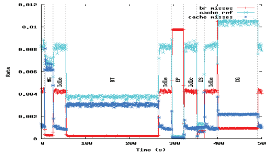
(b) Cache reference and miss rates along with branch miss rate (master node).
